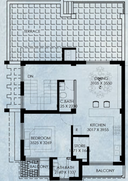
FIRST FLOOR PLAN Total Area : 99.02SQ.M (1065.84SQ.FT)
