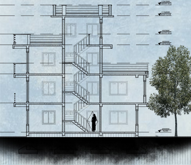
GENERAL SECTION
