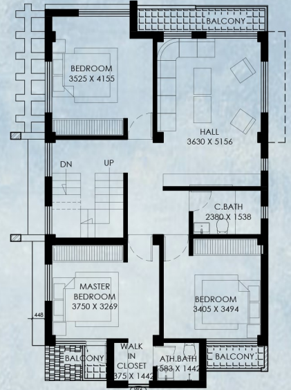
FIRST FLOOR PLAN Total Area : 99.02SQ.M (1065.84SQ.FT)
